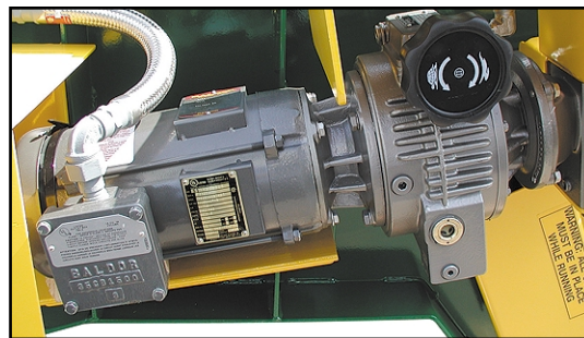
1.5 Horsepower Motor and Variable Speed Drive (remote control available)
