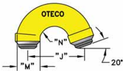
160° Standpipe Gooseneck (GSNK160)
